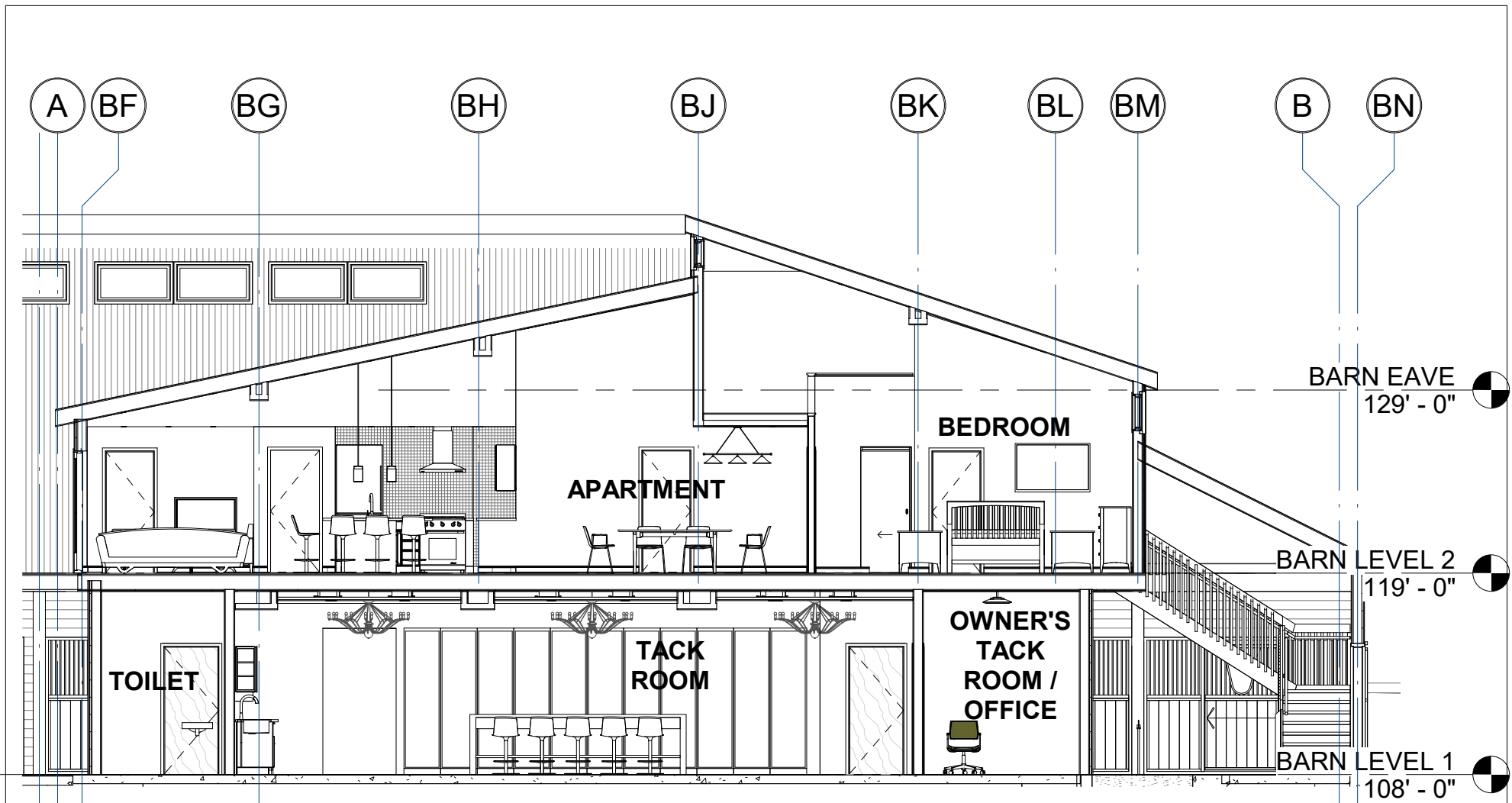
1 PARTIAL BUILDING SECTION 1/8" = 1'-0"
